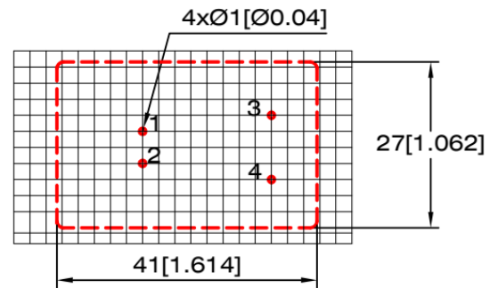
PC Board
